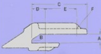
Typical Dimensions
