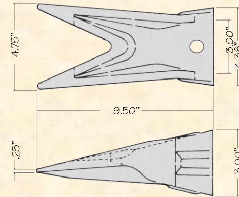
CX-310WT Twin Tiger 12.6#
