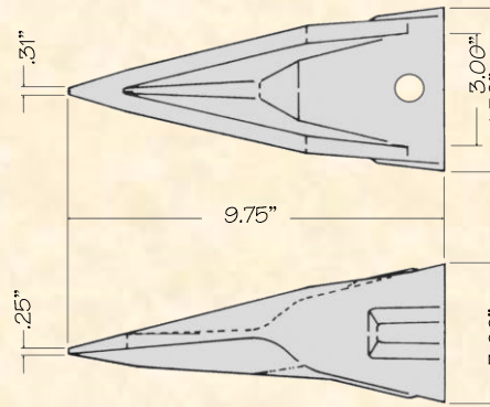
CX-310T Single Tiger 10.7#
