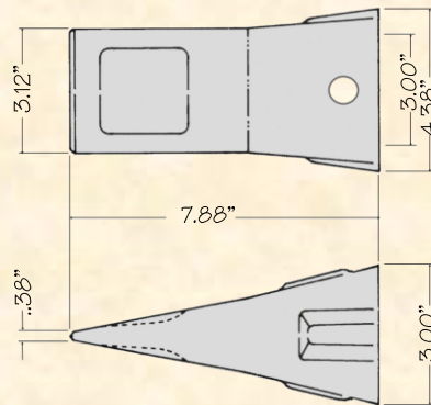
CX-310SP Sharp Penetration 9.5#
