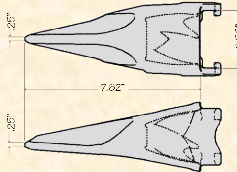
CV-19T Single Tiger Sharp (Same as V19VY) 4.7#
