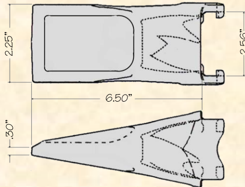
CV-19 General Purpose 5.5#
