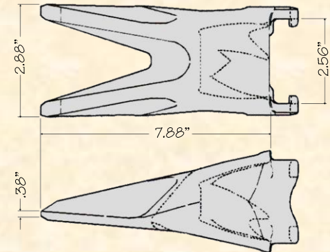
CV-19TT Twin Tiger Sharp (Same as V19TVY) 5.8#
