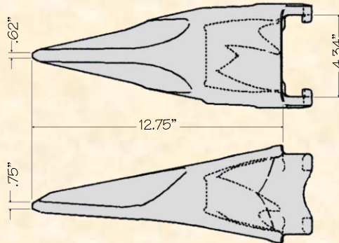
CV-43T Single Tiger Sharp (Same as V43VY) 28.3#
