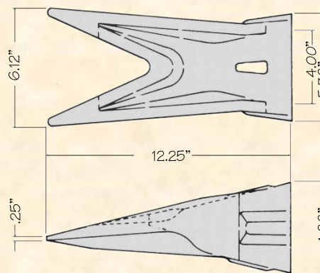
CX-400WT Twin Tiger 24.5#
