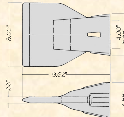
CX-400F Flared Tooth 18.5#
