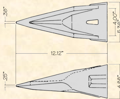
CX-400T Single Tiger 17.5#
