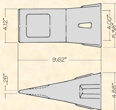
CX-400SP Sharp Penetration 16.0#
