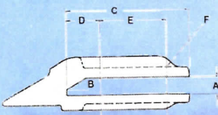
#1A Bolt-on Style Adapter
