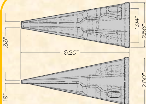
201RE9 Single Sharp
