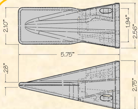
201RE2D Dual Purpose
