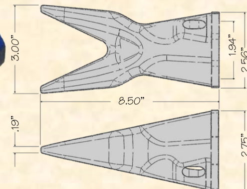
201RE7 Twin Sharp
