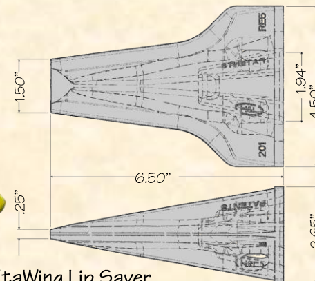
201RE5 DeltaWing Lip Saver
