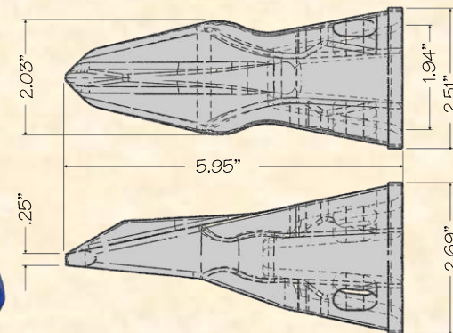
201RE4 Star Penetration
