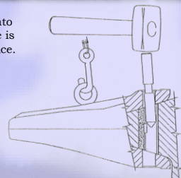
Position one of the “VP” style Series Mining tooth on the adapter nose.
