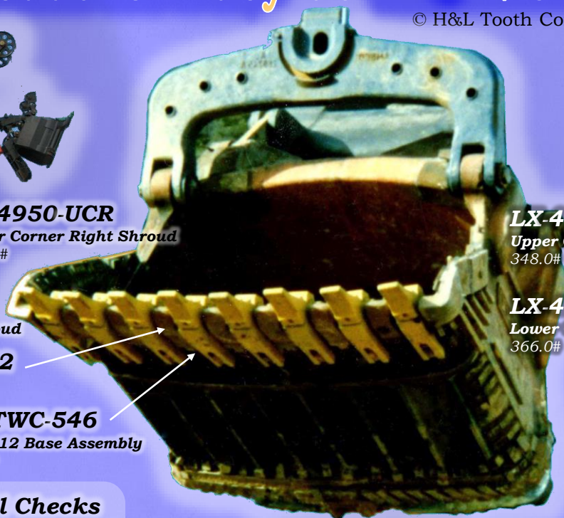
LX-4950-LCL LX-4950-LCR Lower Corner Left & Right
