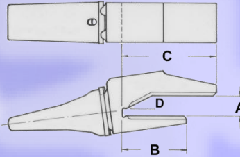
“1W” Loader Adapter
