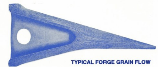
TYPICAL FORGE GRAIN FLOW
