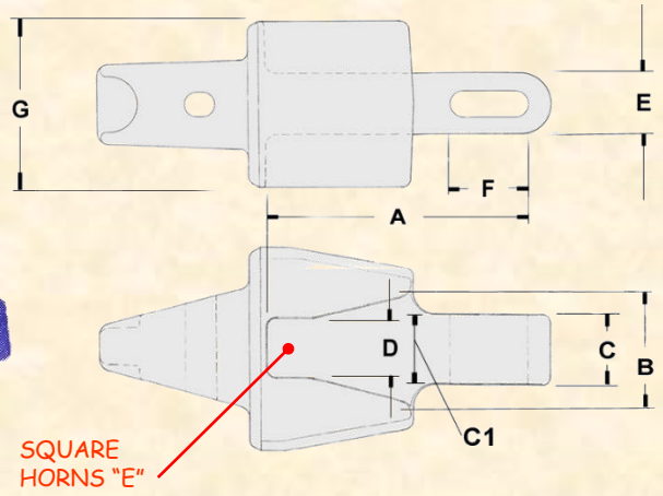
Typical Dimensional layout
