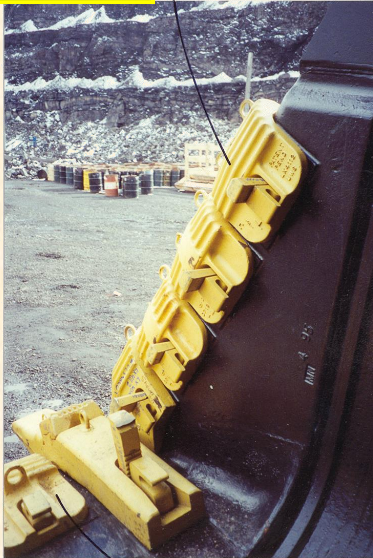
LX-4112 Center Shroud, K-1328 Key with Safety Cap and K-1327 Clamp
