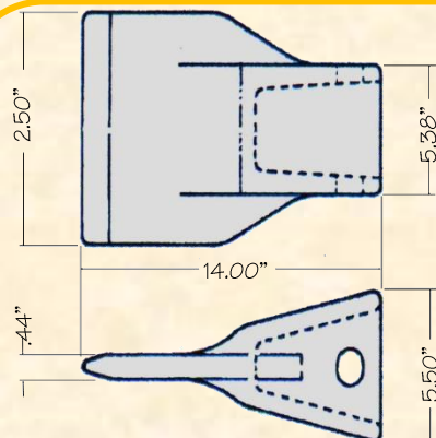
CX-107-3550 Flared Tooth
