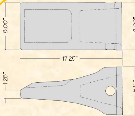
HL-4T-4703 Heavy Abrasion
