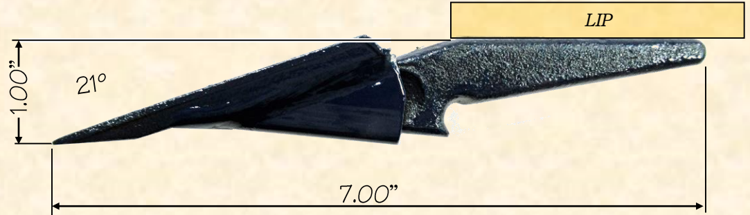
D-842-00SP Assembly at MAXIMUM Digging Depth
