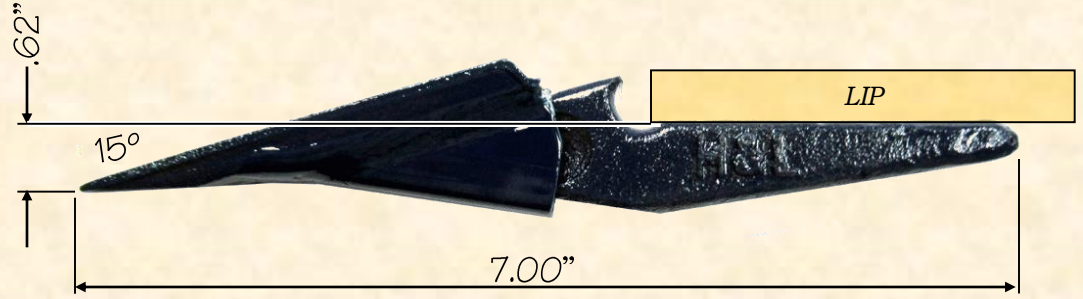
D-842-00SP Assembly at MINIMUM Digging Depth
