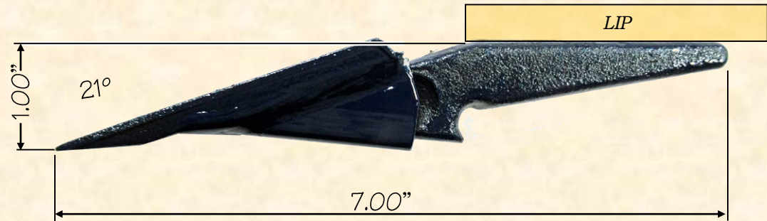
D-872-00SP Assembly at MAXIMUM Digging Depth
