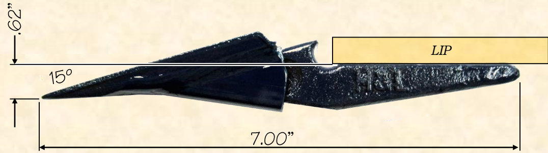
D-872-00SP Assembly at MINIMUM Digging Depth
