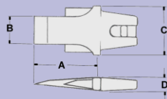
Tooth Dimensions Style 1
