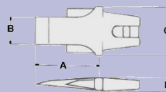
Tooth Dimensions Style 1
