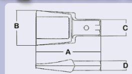
Tooth Dimensions Style 3
