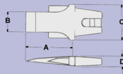
Tooth Dimensions Style 1
