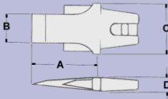
Tooth Dimensions Style 1
