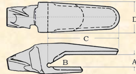
Cobra Line 1W super twist Style Adapter
