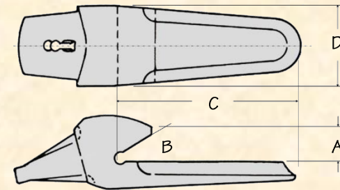
Cobra Line 1CW conical Style Adapter
