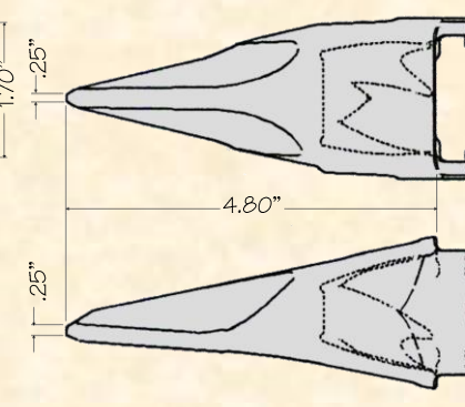
CV-13T Single Tiger Sharp 1.8#
