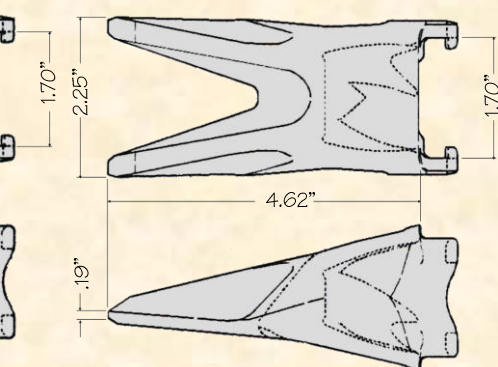
CV-13TVY Twin Tiger Sharp 1.8#
