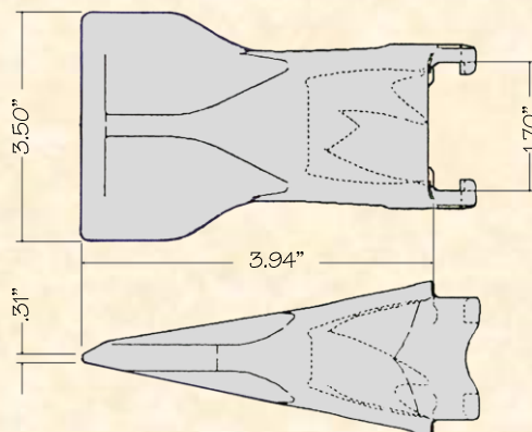
CV-13F Flared Tooth 2.2#
