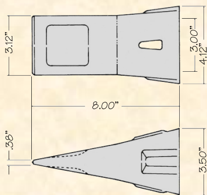
CX-290SP Sharp Penetration 8.2#
