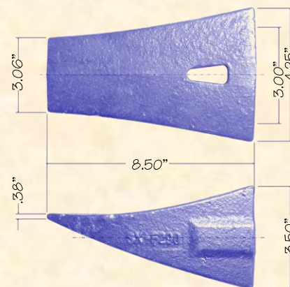
CX-290TF Flange Tooth 11.6#
