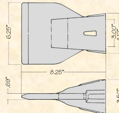
CX-290F Flared Tooth 11.6#
