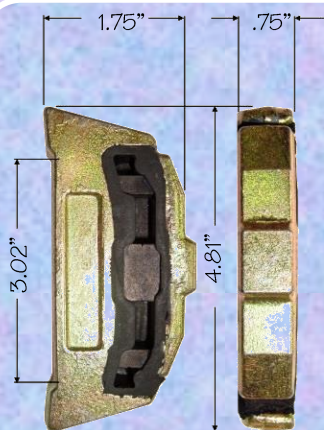
C-475PN
