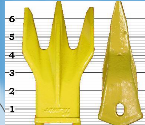
Patented Triple Tiger® Design Uses 23ODFP
